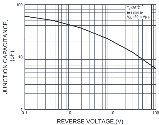
FIG.5-TYPICAL JUNCTION CAPACITANCE
