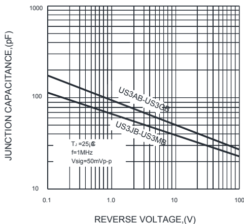
FIG.5-TYPICAL JUNCTION CAPACITANCE
